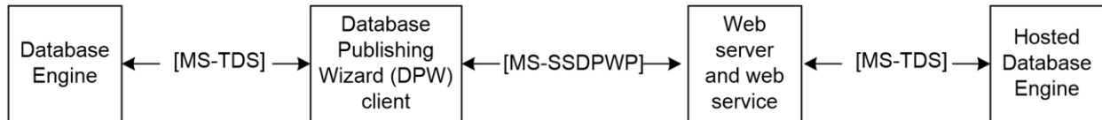
Figure 9: Manageability architecture
