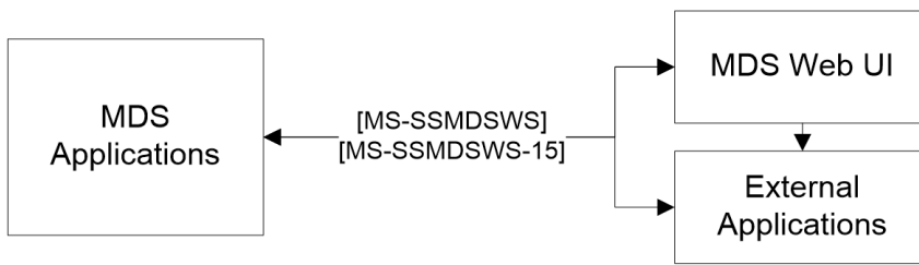
Figure 3: MDS architecture
