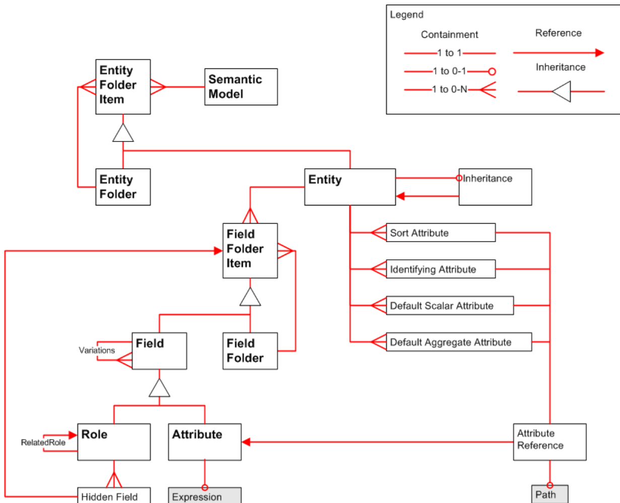
Figure 2: Semantic Objects
