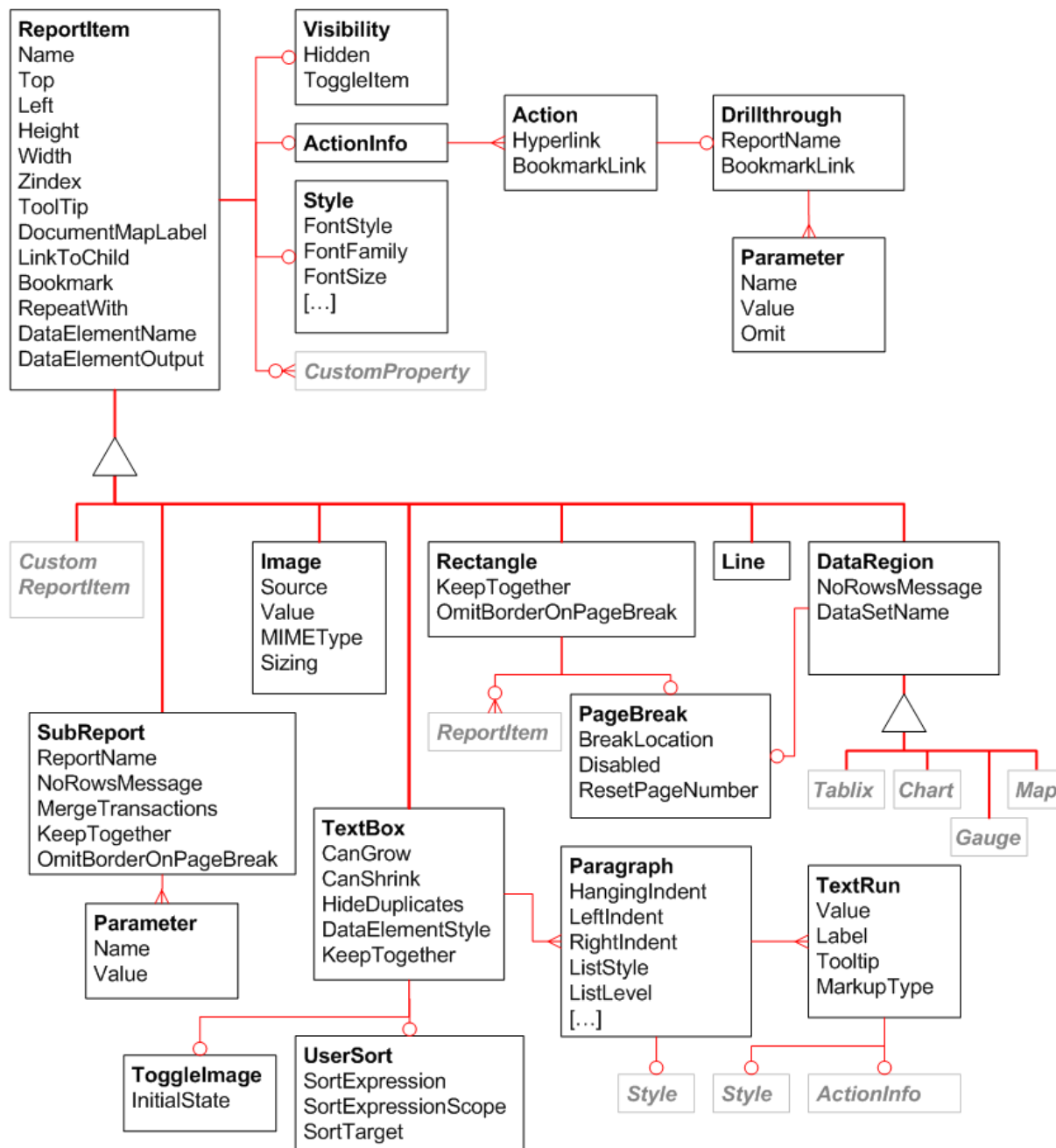
Figure 3: Report items
