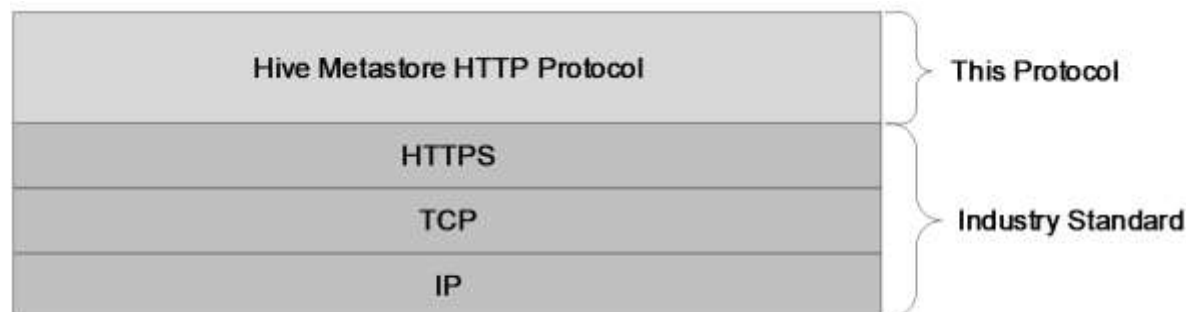
Figure 2: Protocol layering
